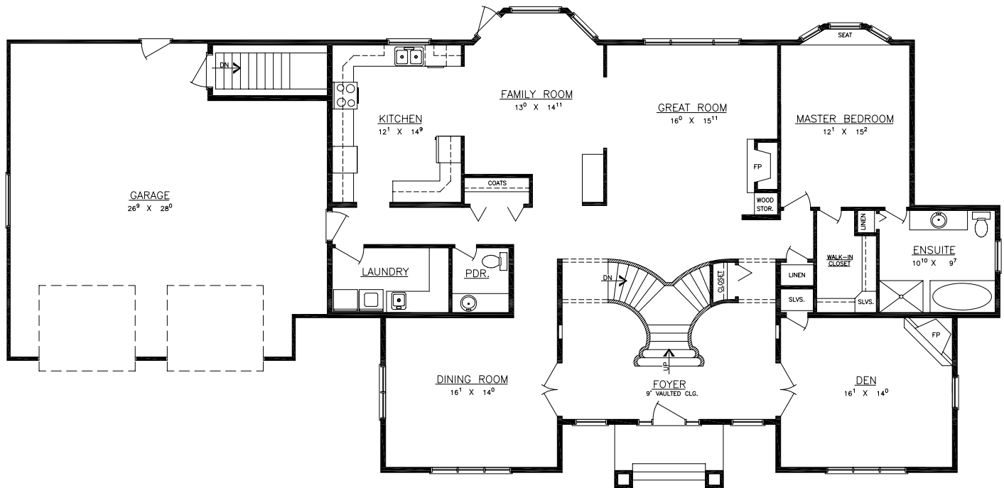
MAIN FLOOR
